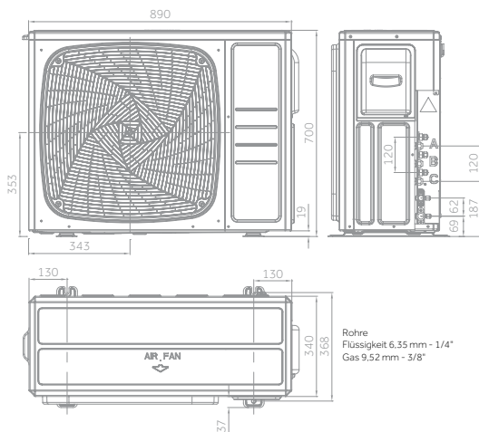
3U55S2SR5FA – 3U70S2SR5FA (3 Kupplungen)
