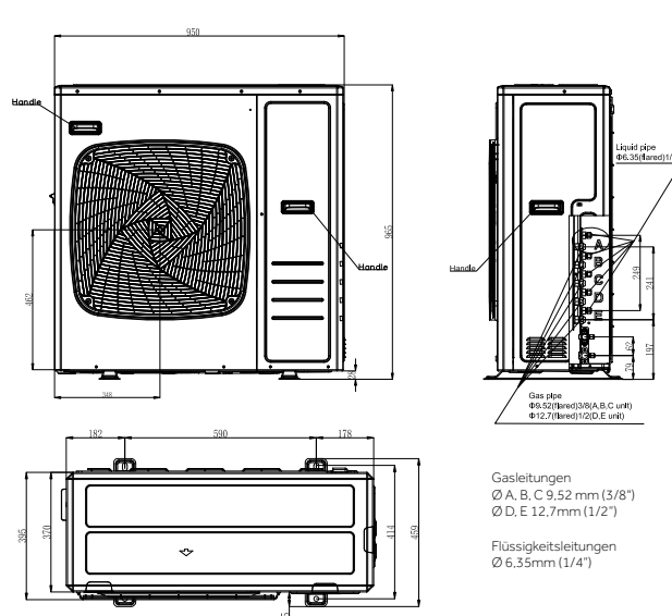
5U125S2SN1FA (5 Anschlüsse)
