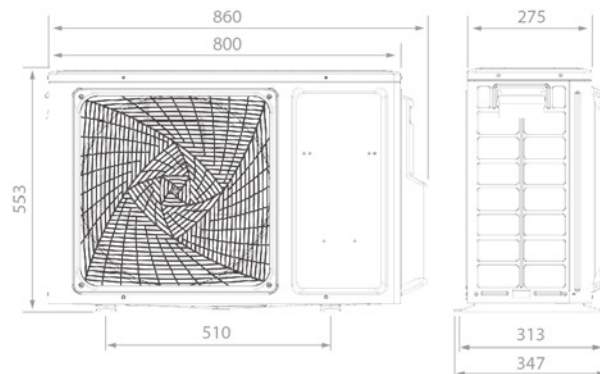
2U50S2SM1FA-3 (2 Anschlüsse)
